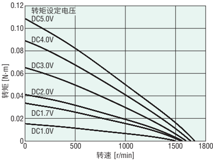
2TK3GN-AW2U、2TK3A-AW2U (115V 60Hz)
