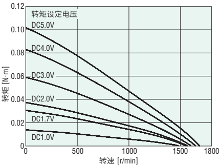
2TK3GN-AW2U、2TK3A-AW2U (110V 60Hz)
