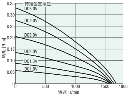
4TK10GN-CW2E、4TK10A-CW2E (220V 50Hz) 4TK10GN-CW2E、4TK10A-CW2E (220V 60Hz)
