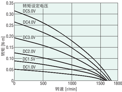
4TK10GN-AW2U、4TK10A-AW2U (115V 60Hz)
