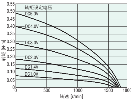
5TK20GN-AW2U、5TK20A-AW2U (115V 60Hz)
